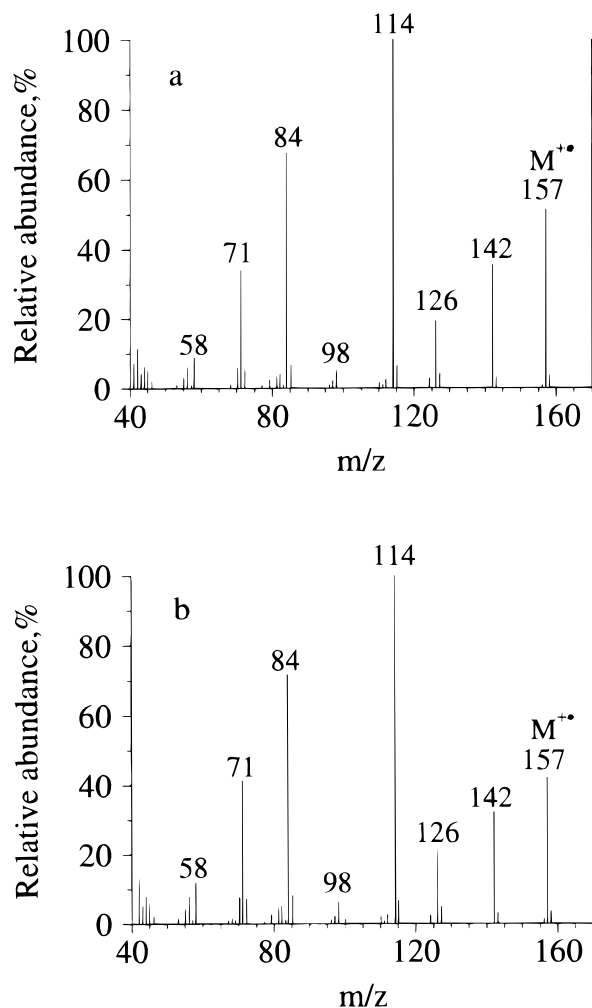
Figure 4. EI mass spectra of stereoisomeric 1-methoxy-3-dimethylaminocyclohexanes cis - and trans -5.
