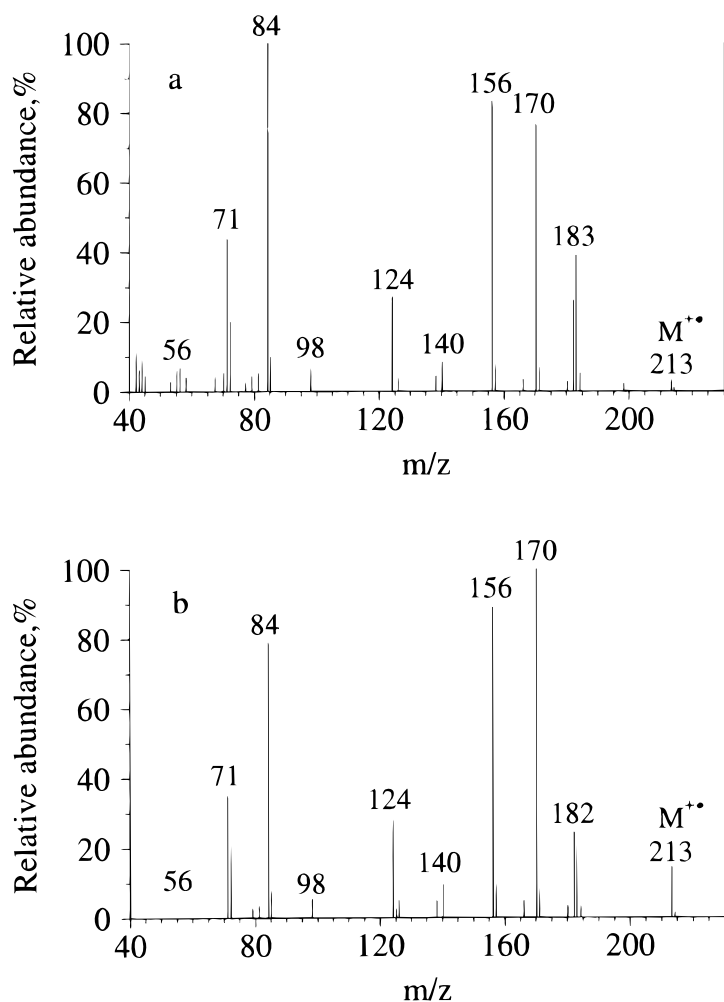
Figure 2. EI mass spectra of stereoisomeric 1-butyl-1-methoxy-3-dimethylaminocyclohexanes cis - and trans -3 (R = C 4 H 9 ).
