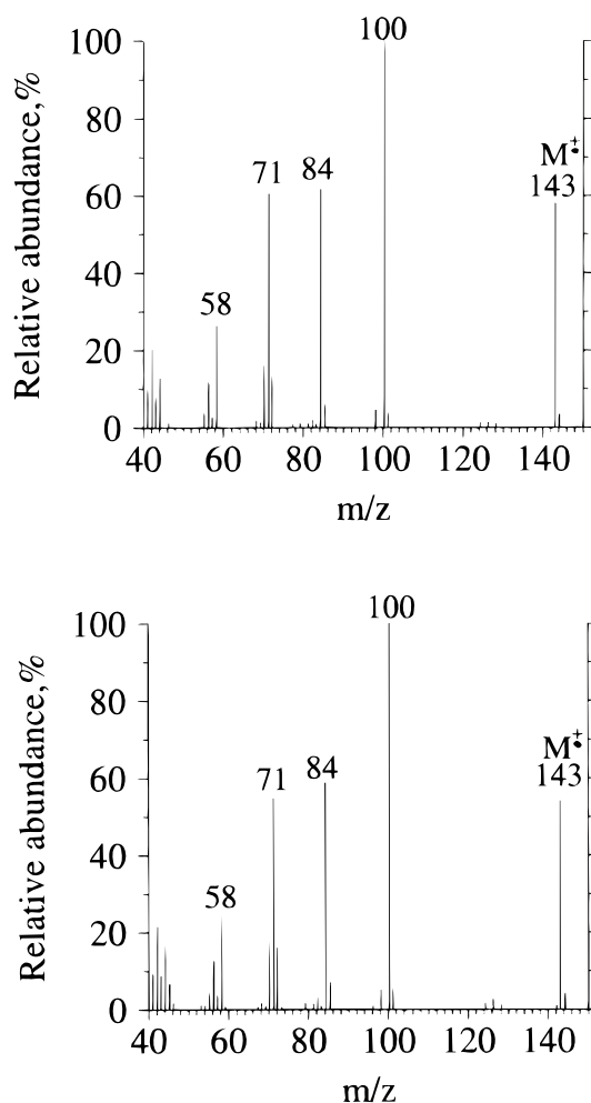
Figure 3. EI mass spectra of stereoisomeric unsubstituted 3-dimethylaminocyclohexanes cis - and trans -4.
