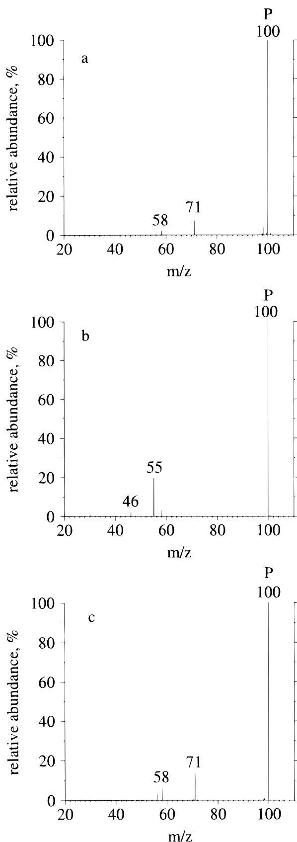
Figure 1. CID spectra of m/z 100 ions: (a) obtained from cis -1-butyl-3-dimethylaminocyclohexanol ( cis -1, R = C_4H_9 ) under 70 eV EI conditions; (b) protonated (isobutane CI) dimethylaminocyclobutane (ion a); (c) CID spectrum of m/z 100 ion b obtained from 4-dimethylaminoheptane (2) upon EI.
